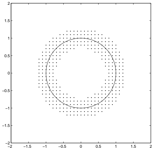
Figure 1: Underlying computational grid for the unit circle. This example corresponds to a mesh spacing of \Delta x = 0.1 and degree-two interpolation polynomials with a five point differencing stencil.
