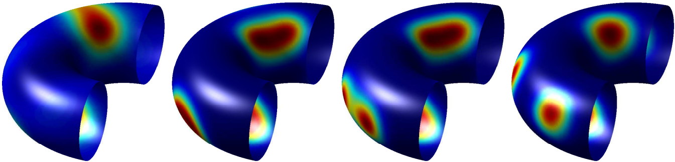
Figure 4: Schnakenberg system evolving on a U-shaped tube. The activator u is displayed at times t = 0.01, 0.03, 0.05, 0.13 . This simulation takes \Delta t = 1.5625e - 07, \Delta x = 1/160 and uses an analytical representation of the closest point to the tube. Forward Euler time-stepping and degree-three interpolating polynomials are used throughout the calculation.
