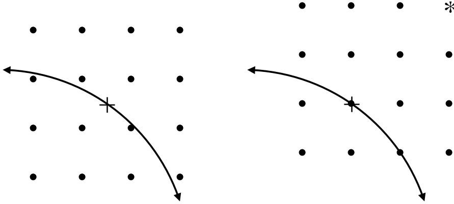
Figure 2: Interpolation stencil corresponding to degree-three interpolation polynomials for a point “+”. Left: From a bandwidth perspective, the grid is optimal for interpolating at the point in question since no stencil node lies more than a distance 1.5\sqrt{2}\Delta x from the interpolation point. Right: For this grid the most symmetrical interpolation stencil will have some grid point “*” a distance 2\sqrt{2}\Delta x from the interpolation point. The bandwidth will be determined by the distance from the interpolation point to the nearest neighbors of “*”.
