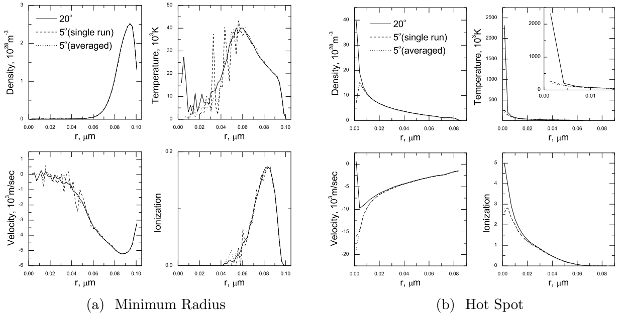
Fig. 5. Systematic vs. Statistical error. The jitter in the first figure is due to the statistically small number of atoms, and can be effectively eliminated by averaging over several runs. The second figure demonstrates systematic error introduced by the cone.
