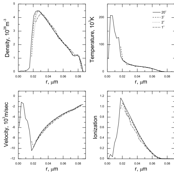
Fig. 7. Very small angles. The snapshot is taken at an intermediate radius, same as in Figure 3(b). The graphs for small angles are missing points near the center due to a very low number of particles there.
