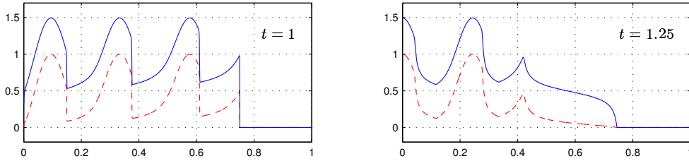
Figure 17: Dissolved concentration u (dashed lines) and total concentration u + v (solid lines) for the adsorption-desorption problem at time t = 1 (left) and t = \frac{5}{4} (right).
