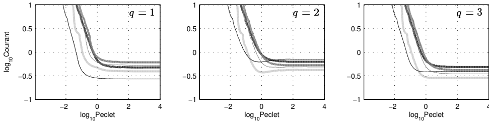
Figure 5: Boundaries of \mathcal{D}_{AD}(q) for the third-order methods IMEX-BDF3 (dark gray), IMEX-TVB(3,3) (gray), IMEX-Shu(4,3) (light gray), IMEX-Shu(5,3) (thin gray) and IMEX-Adams3 (thin black).
