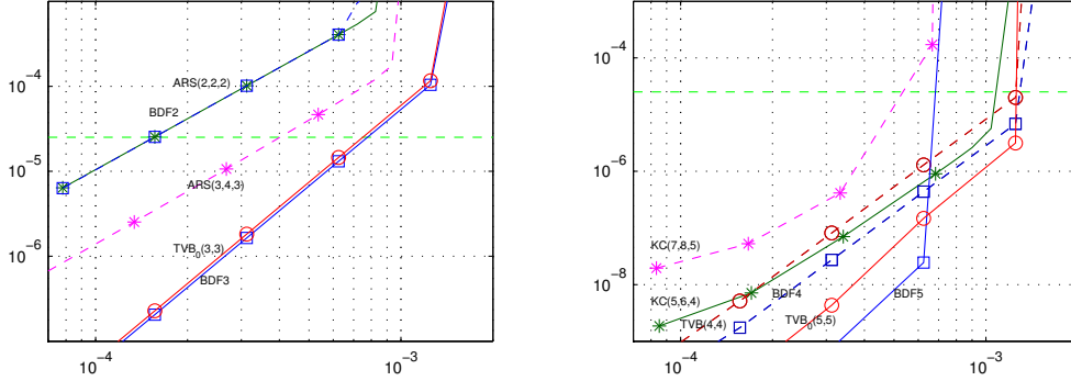
Figure 16: Temporal L_1 -errors vs. scaled step sizes, m = 400 , spatial error 1.5 \times 10^{-5} . Left: second- and third-order methods ARS(2,2,2), ARS(3,4,3), IMEX-BDF2, IMEX-BDF3 and IMEX-TV B_0 (3,3). Right: high-order methods KC(5,6,4), KC(7,8,5), IMEX-BDF4, IMEX-BDF5, IMEX-TV B_0 (4,4) and IMEX-TV B_0 (5,5). Marker * for the IMEX Runge-Kutta methods, \square for the IMEX-TV B_0 methods and \circ for the IMEX-BDF methods.
