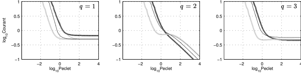
Figure 3: Boundaries of \mathcal{D}_{AD}(q) , q = 1, 2, 3 , for the second-order methods IMEX-BDF2 (dark gray), IMEX-Adams2 (thin black) and the IMEX-Shu(3,2) extensions (3.4) (light gray) and (3.5) (thin gray; largely coinciding with the light gray line for large \mu and the dark gray line for small \mu .)
