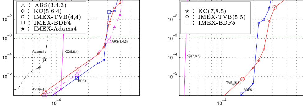
Figure 19: Temporal L_1 -errors vs. scaled step sizes \in (4 \times 10^{-5}, 6 \times 10^{-4}) , m = 800 , spatial error 1.2 \times 10^{-3} . Left: fourth-order methods KC(5,6,4), IMEX-BDF4, IMEX-TVB(4,4) and IMEX-Adams4. For comparison, results of the third-order method ARS(3,4,3) are added. Right: fifth-order methods KC(7,8,5), IMEX-BDF5 and IMEX-TVB 0 (5,5). Markers for KC(7,8,5) are outside the displayed range.
