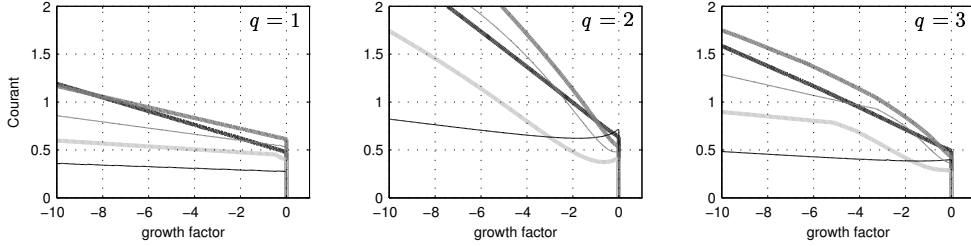
Figure 4: Boundaries of \mathcal{D}_{AR}(q) for the third-order methods IMEX-BDF3 (dark gray), IMEX-TVB(3,3) (gray), IMEX-Shu(4,3) (light gray), IMEX-Shu(5,3) (thin gray) and IMEX-Adams3 (thin black).
