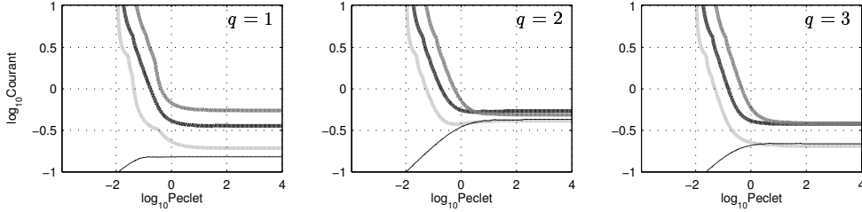
Figure 7: Boundaries of \mathcal{D}_{AD}(q) for the fourth-order methods IMEX-BDF4 (dark gray), IMEX-TVb(4,4) (gray), IMEX-Shu(6,4) (light gray) and IMEX-Adams4 (thin black).
