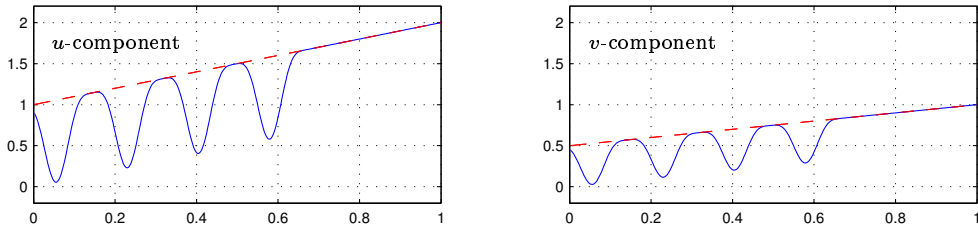
Figure 15: Components u (left) and v (right) at t = 1 for the linear advection-reaction problem with \gamma_1(t) = 1 - \sin(12t)^4 . The initial solutions are indicated by dashed lines.
