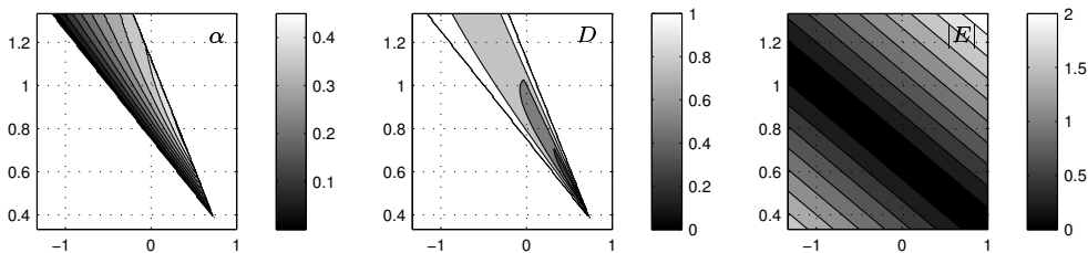
Figure 1: Estimated angles \alpha , damping factors D and absolute error constants |E| for (3.3), with parameter b_0 \in [\frac{1}{3}, \frac{4}{3}] on the vertical axis and b_1 \in [-\frac{4}{3}, 1] horizontally.
