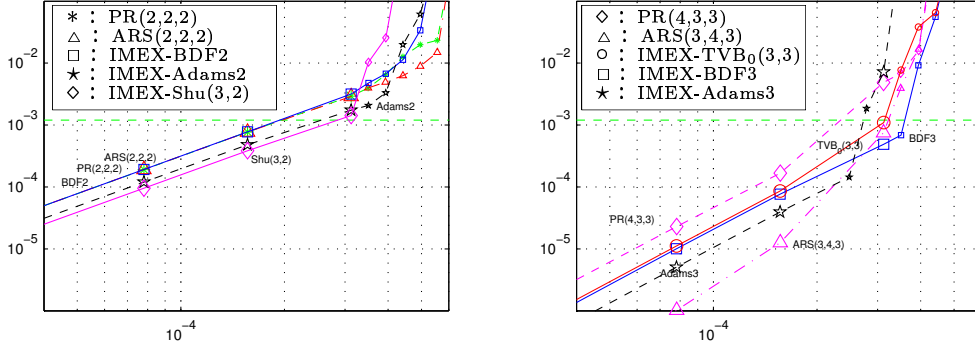
Figure 18: Temporal L_1 -errors vs. scaled step sizes \in (4 \times 10^{-5}, 6 \times 10^{-4}) , m = 800 , spatial error 1.2 \times 10^{-3} . Left: second-order methods ARS(2,2,2), PR(2,2,2), IMEX-BDF2, IMEX-Adams2 and IMEX-Shu(3,2). The results for ARS(2,2,2), PR(2,2,2), IMEX-BDF2 are virtually the same for small step sizes. Right: third-order methods ARS(3,4,3), PR(4,3,3), IMEX-BDF3, IMEX-TVB 0 (3,3) and IMEX-Adams3.
