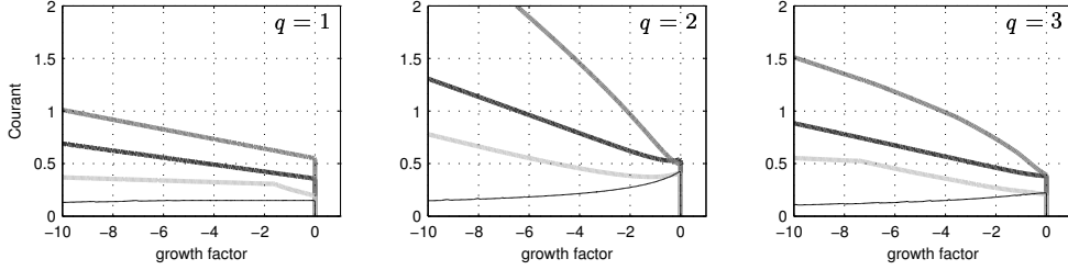
Figure 6: Boundaries of \mathcal{D}_{AR}(q) for the fourth-order methods IMEX-BDF4 (dark gray), IMEX-TVb(4,4) (gray), IMEX-Shu(6,4) (light gray) and IMEX-Adams4 (thin black).
