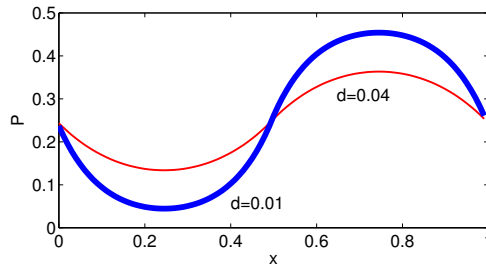
Figure 12: Steady state population density for the population dynamics model with diffusion constants d = 0.01 and d = 0.04 .
