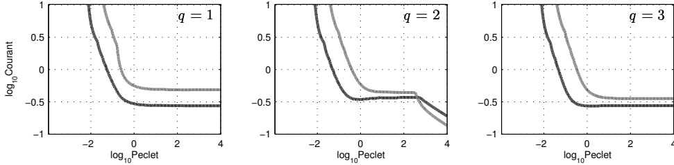
Figure 9: Boundaries of \mathcal{D}_{AD}(q) for the fifth-order methods IMEX-BDF5 (dark gray) and IMEX-TVB 0 (5,5) (gray).
