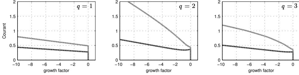
Figure 8: Boundaries of \mathcal{D}_{AR}(q) for the fifth-order methods IMEX-BDF5 (dark gray) and IMEX-TVB 0 (5,5) (gray).
