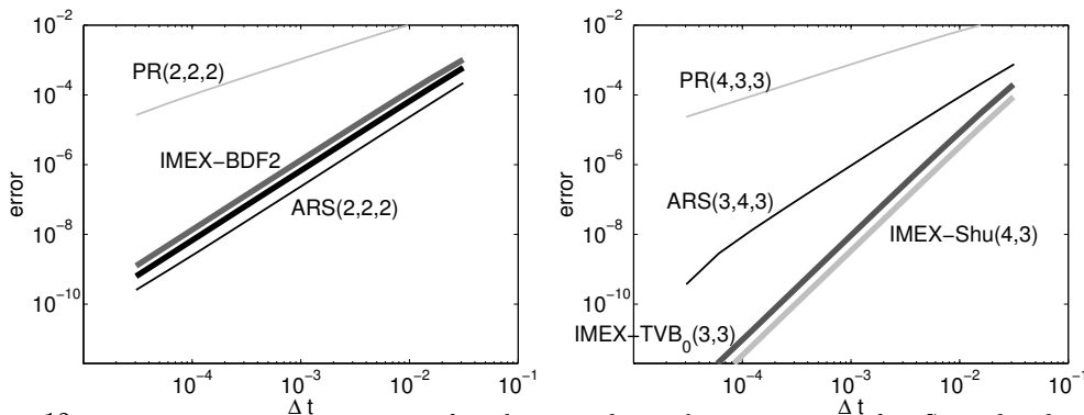
Figure 13: Errors vs. scaled step size for the van der Pol equation. Left: Second-order methods. The thick black line (unlabeled to avoid cluttering the plot) corresponds to IMEX-Shu(3,2) and IMEX-SG(3,2). The IMEX-Adams2 results lie midway between those for IMEX-Shu(3,2) and IMEX-TVB 0 (3,3). Right: Third-order methods. IMEX-BDF3 essentially overlaps the results for IMEX-TVB 0 (3,3). IMEX-Shu(5,3) and IMEX-Adams3 results lie between the results for IMEX-TVB 0 (3,3) and IMEX-Shu(4,3).
