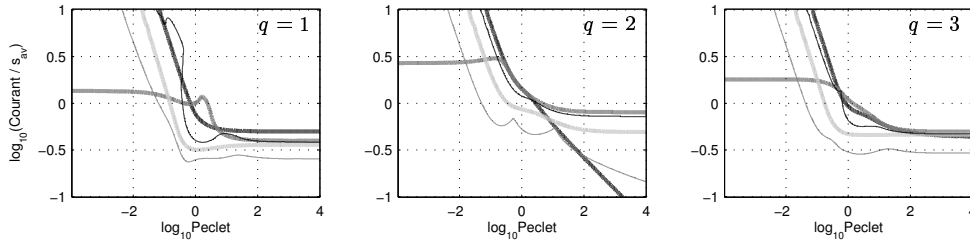
Figure 11: Boundaries of scaled domains \mathcal{D}_{AD}(q) for the IMEX Runge-Kutta methods PR(2,2,2) (dark gray), ARS(3,4,3) (gray), PR(4,3,3) (light gray), KC(5,6,4) (thin black) and KC(7,8,5) (thin gray). The scaled domains for ARS(2,2,2) (not shown) are close to PR(2,2,2).
