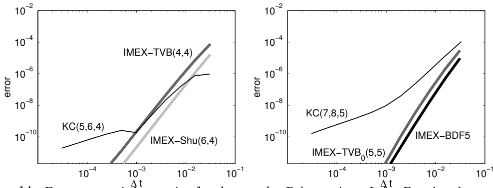
Figure 14: Errors vs. scaled step size for the van der Pol equation. Left: Fourth-order methods. The IMEX-BDF4 results lie midway between IMEX-TV B(4,4) and IMEX-Shu(6,4). Right: Fifth-order methods.
