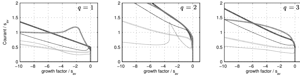
Figure 10: Boundaries of scaled domains \mathcal{D}_{AR}(q) for the IMEX Runge-Kutta methods PR(2,2,2) (dark gray), ARS(3,4,3) (gray), PR(4,3,3) (light gray), KC(5,6,4) (thin black) and KC(7,8,5) (thin gray). The scaled domains for ARS(2,2,2) (not shown) are close to PR(2,2,2).
