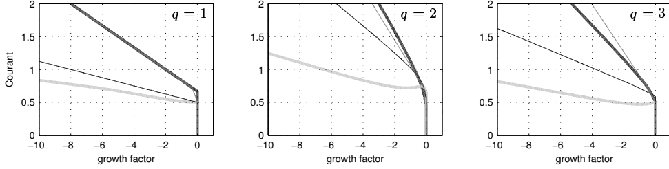
Figure 2: Boundaries of \mathcal{D}_{AR}(q) , q = 1, 2, 3 , for the second-order methods IMEX-BDF2 (dark gray), IMEX-Adams2 (thin black) and the IMEX-Shu(3,2) extensions (3.4) (light gray) and (3.5) (thin gray).
